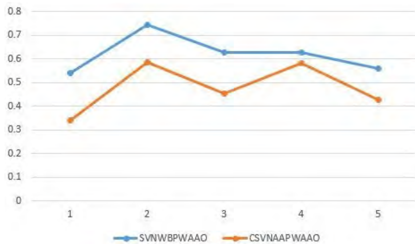
FIGURE 1. Graphical comparison of SVNWPWAAO and CSVNAPWAAO
