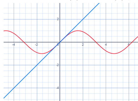
FIGURE 2. \sin(x) = x, \sin(x) \neq x
