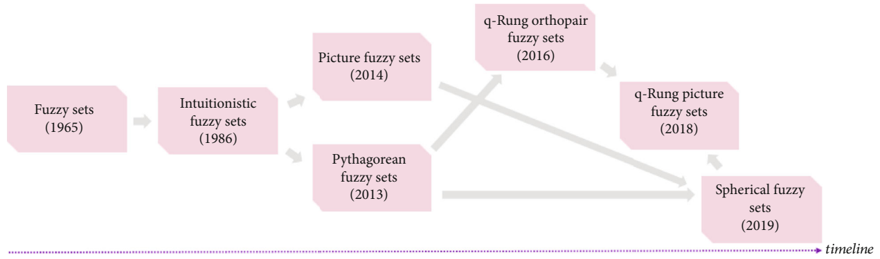
FIGURE 1: Development network of fuzzy set theory.
