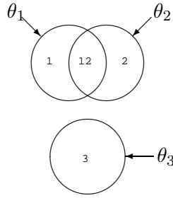
Fig. 3: Venn diagram of a DSMT hybrid model for a 3D frame.
