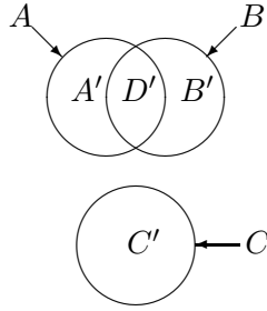
Fig. 4: Hybrid model for \Theta = \{A, B, C\} .
