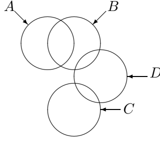
Fig. 6: Venn Diagram for the hybrid model for this example.
