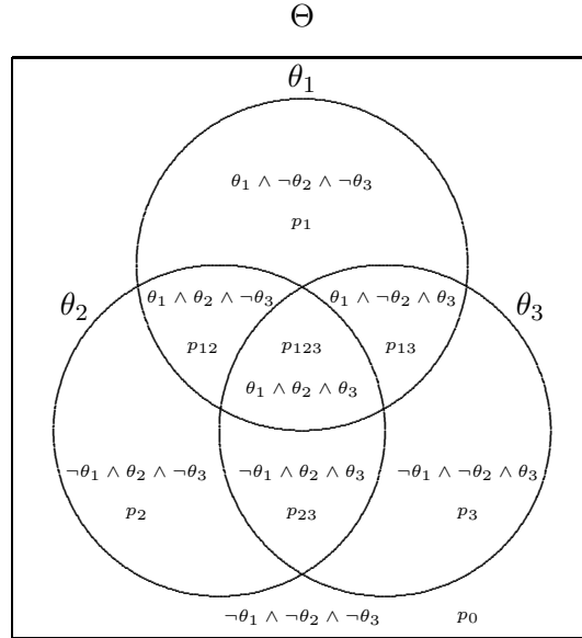
Fig. 2: Venn diagram of the free DSMT model for a 3D frame.
