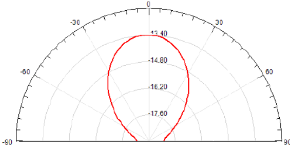
Fig.6. The E-Plane radiation pattern for the antenna at 2.8 GHz when all switches are OFF
