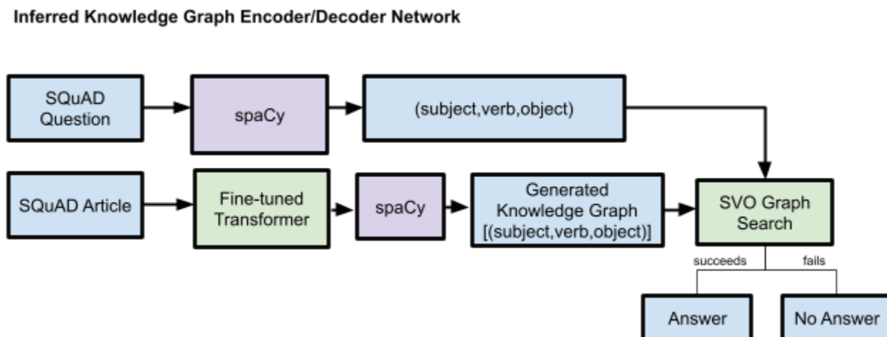
Fig 8. Architecture of experiment, with SVO parsing and inferred knowledge graph generation
