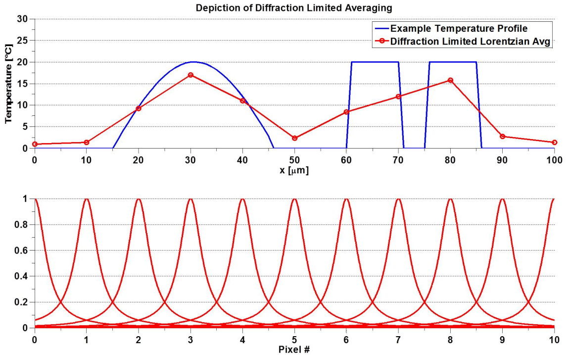
Figure 5.7: Depth averaged Si-microheater line temperature with example diffraction limited pixel temperature (top) and the corresponding spacial Lorentzian pixel weighting functions (bottom).
