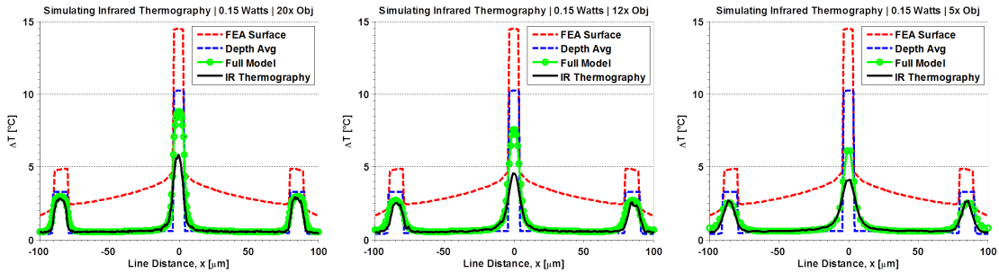
Figure 5.15: FEA surface temperature with full simulation vs measured IR temperature for a power input of 0.15 Watts at various objective magnifications.
