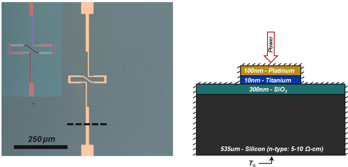
Figure 2.1: a.)Optical image, and b.)Cross-section diagram of the control heater device. Inset of (a) shows false color highlighting individual cuboids used in analysis of heater
