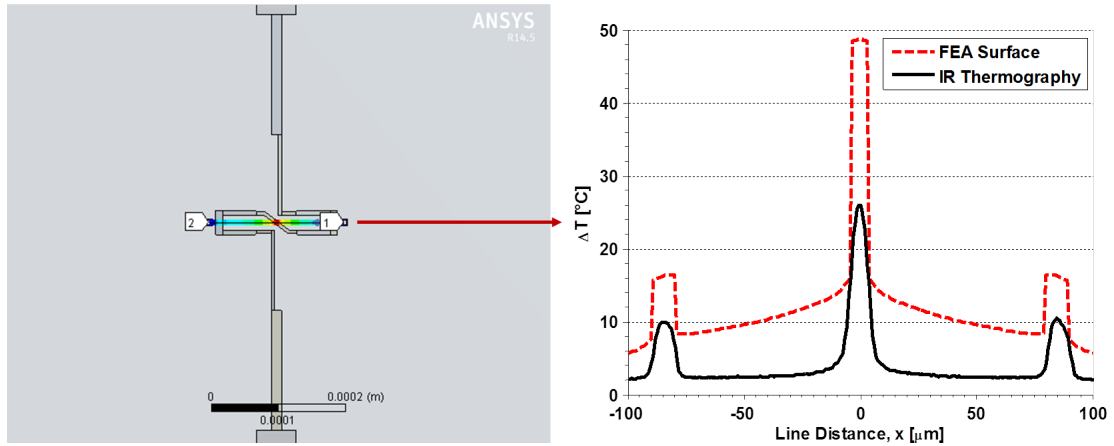
Figure 5.8: b.) FEA surface temperature vs measured IR temperature over the line depicted in (a).
