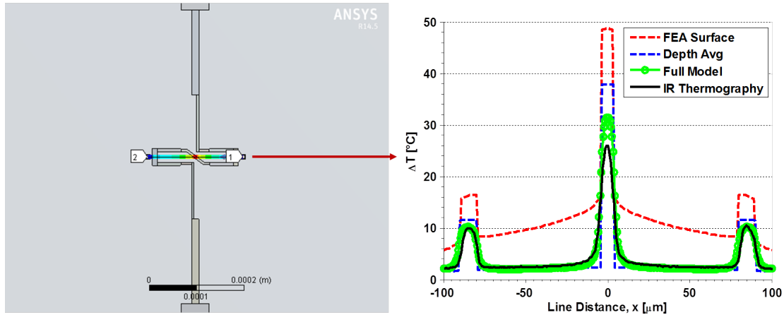
Figure 5.12: b.) FEA surface temperature with full simulation vs measured IR temperature, over the line depicted in (a).
