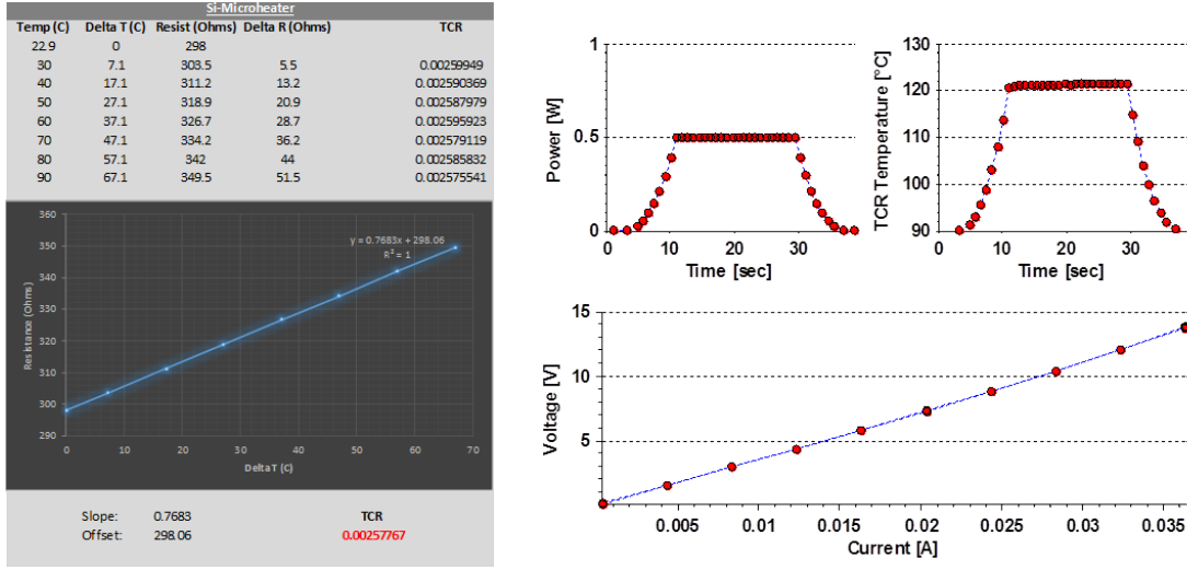
Figure 3.1: a.) Measured device TCR data, and b.) Subsequent TCR temperature of powered device shown in Figure 3.3a.
