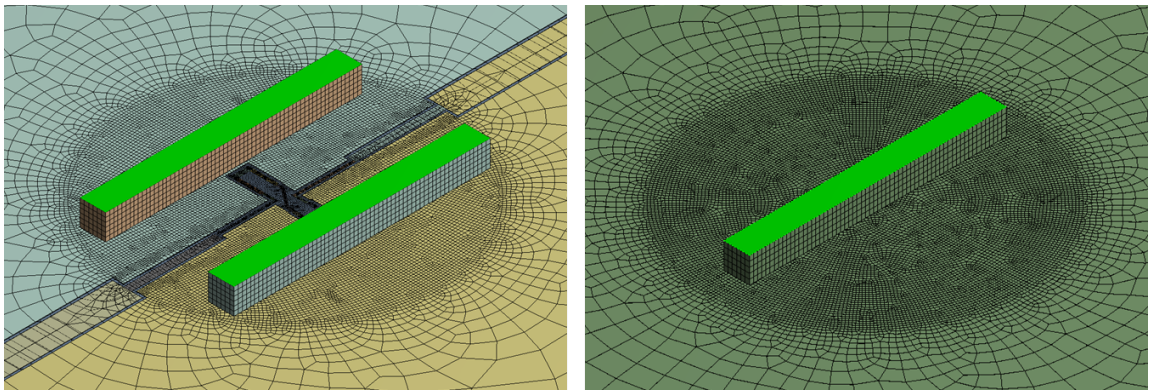
Figure 2.7: Finite element mesh of the topside copper ribbon heat sink
