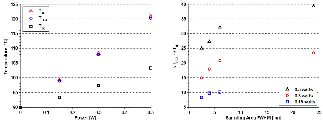
Figure 3.4: (a) Nominal heater temperatures obtained via each thermal characterization technique plotted as a function of power dissipation, and (b) difference in peak temperatures over the dashed lines in Figure 3.3 plotted as a function of measured IR resolution.
