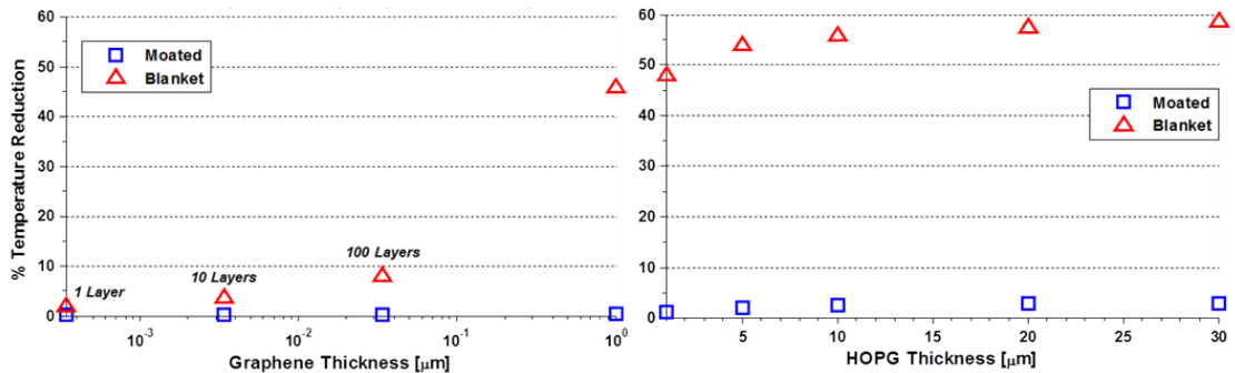
Figure 4.2: Cooling capability of a.) graphene and b.) graphite as a function of layer thickness.
