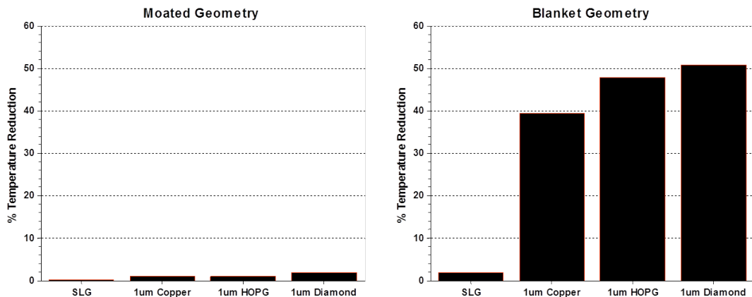
Figure 4.1: Top-side heat spreader simulation results
