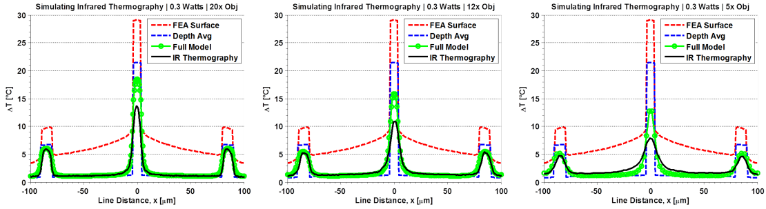
Figure 5.14: FEA surface temperature with full simulation vs measured IR temperature for a power input of 0.3 Watts at various objective magnifications.
