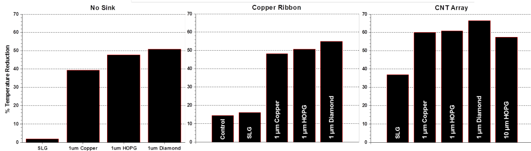
Figure 4.3: a.) 2-way stand-alone heat-spreader simulation results, b.) 3-way copper ribbon heat-sink simulation results, and c.) 3-way CNT array heat-sink simulation results
