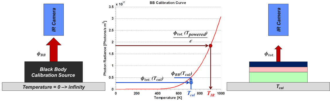
Figure 5.5: Diagram depicting an IR thermography procedure using Eq 5.8 and 5.33
