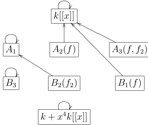
Figure 4.17: Diagram of \star_{B_1(f_1)} \cap \star_{A_1} , auxiliary slice.
