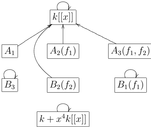
Figure 4.20: Diagram of \star_{B_1(f_1)} , main slice.
