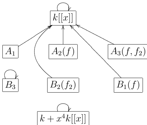
Figure 4.8: Diagram of \star_{B_1(f_1)} , auxiliary slice.
