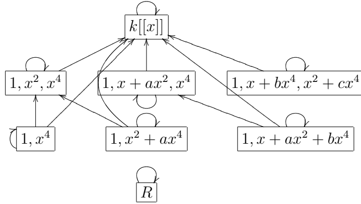
Figure 5.1: All possible actions of star operations on R = k[[x^3, x^5, x^7]] .
