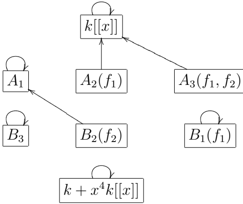
Figure 4.16: Diagram of \star_{B_1(f_1)} \cap \star_{A_1} , main slice.
