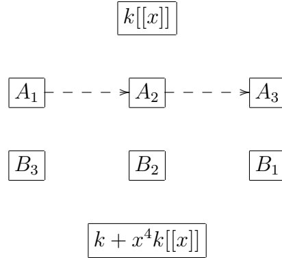
Figure 3.2: Implication by Proposition 3.0.14 applied to k + x^4 k[[x]] .
