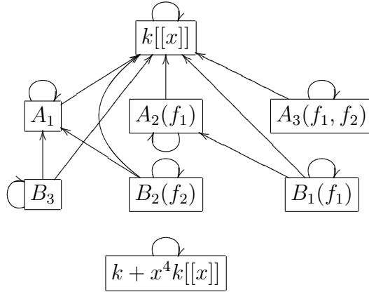
Figure 3.3: All possible actions of star operations on k + x^4k[[x]] .
