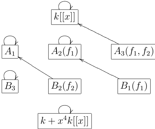
Figure 4.2: Diagram of \star_{B_3} .
