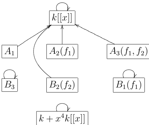
Figure 4.7: Diagram of \star_{B_1(f_1)} , main slice.
