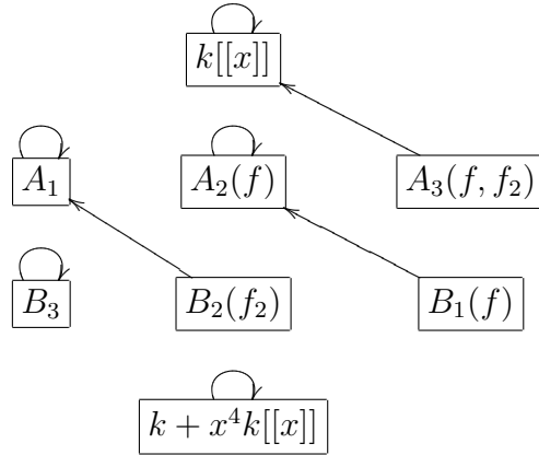
Figure 4.10: Diagram of \star_{B_3} \cap \star_{B_1(f_1)} , auxiliary slice.
