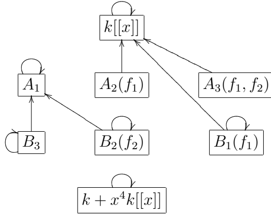
Figure 4.11: All possible actions of star operations on k + x^4k[[x]] assuming that A_1^* = A_1 and A_2^* = k[[x]] .
