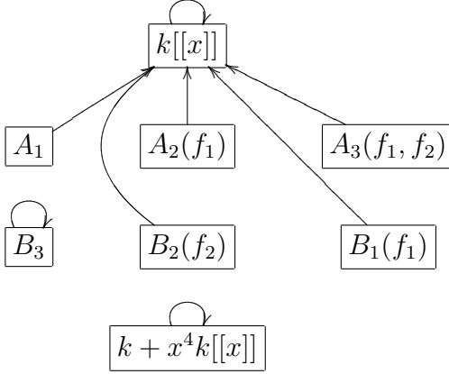
Figure 4.15: Diagram of \star_{B_3} \oplus \star_{B_1} .
