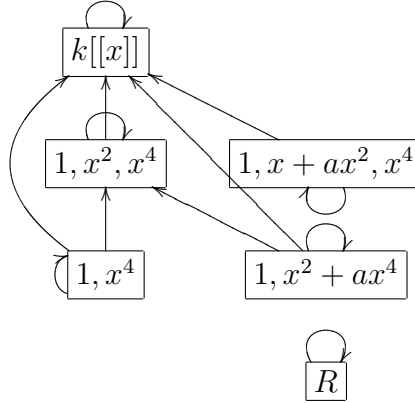
Figure 5.2: All possible actions of star operations on R = k[[x^3, x^5, x^7]] revised.
