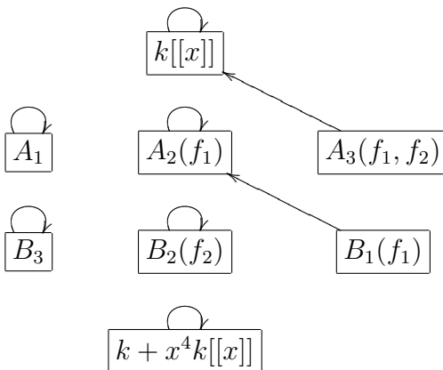
Figure 4.5: Diagram of B_3 \cap B_2(f_2) , main slice.
