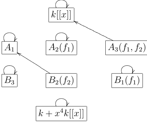
Figure 4.9: Diagram of \star_{B_3} \cap \star_{B_1(f_1)} , main slice.
