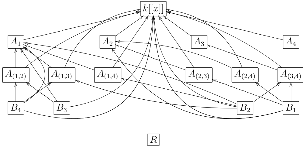
Figure 5.3: All possible star operations on k + x^5k[[x]] .
