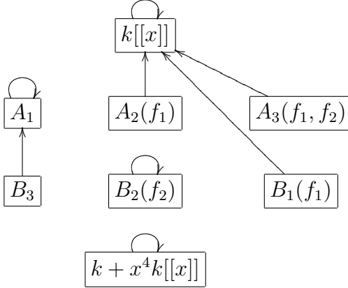
Figure 4.13: Diagram of \star_{B_2(f_2)} \cap \star_{A_1} , main slice.
