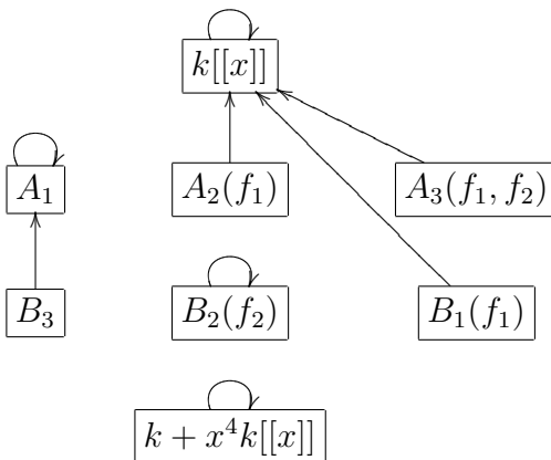
Figure 4.3: Diagram of \star_{B_2(f_2)} , main slice.
