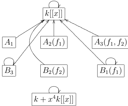
Figure 4.18: All possible actions of star operations on k + x^4k[[x]] assuming that A_1^\star = A_2^\star = k[[x]] .
