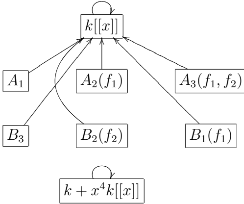
Figure 4.19: Diagram of the v -operation on k + x^4k[[x]] .
