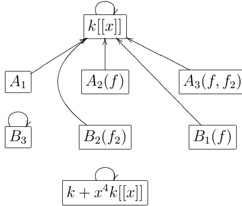
Figure 4.21: Diagram of \star_{B_1(f_1)} , auxiliary slice.
