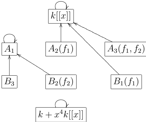
Figure 4.12: Diagram of \star_{A_1} = \star_{B_3} \oplus \star_{B_2} .
