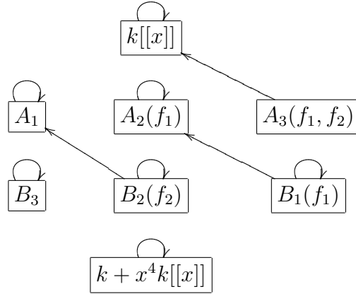
Figure 4.1: All possible star operations on k + x^4k[[x]] assuming A_1 and A_2 are \star -closed.
