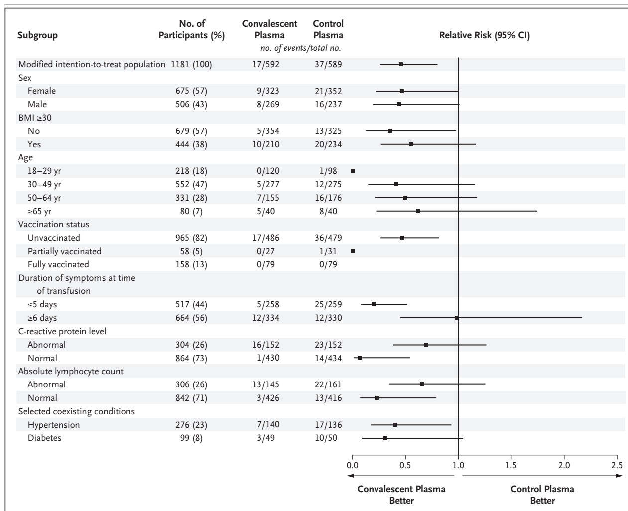
Figure 3. Subgroup Analyses.
