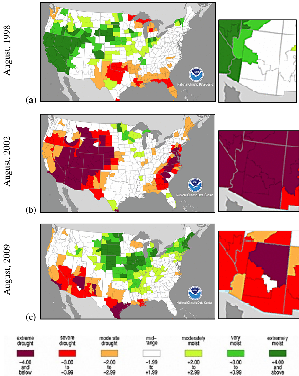
Figure 3. Palmer Drought Severity Index (PDSI) by NOAA in Arizona: a) Aug. 1998, b) Aug. 2002, and c) Aug. 2009. Color scheme: maroon (-4.0 or below) extreme drought, orange (-2 to -2.9) moderate drought, white (-1.9 to +1.9) near normal, light green (+3.0 to +3.9) very moist, and dark green (+4.0 and above) extremely moist.
