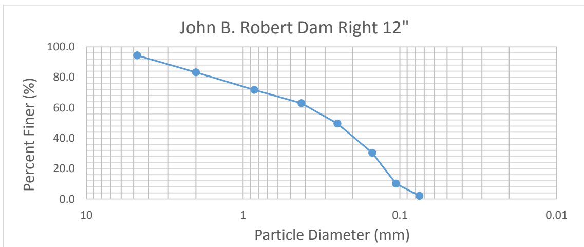
Figure 44: 12" Right Location - Sieve Analysis JBR Dam
