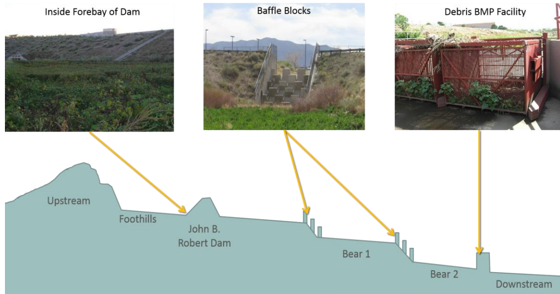
Figure 8: Schematic of sites within the Bear Arroyo watershed and water quality structure locations
