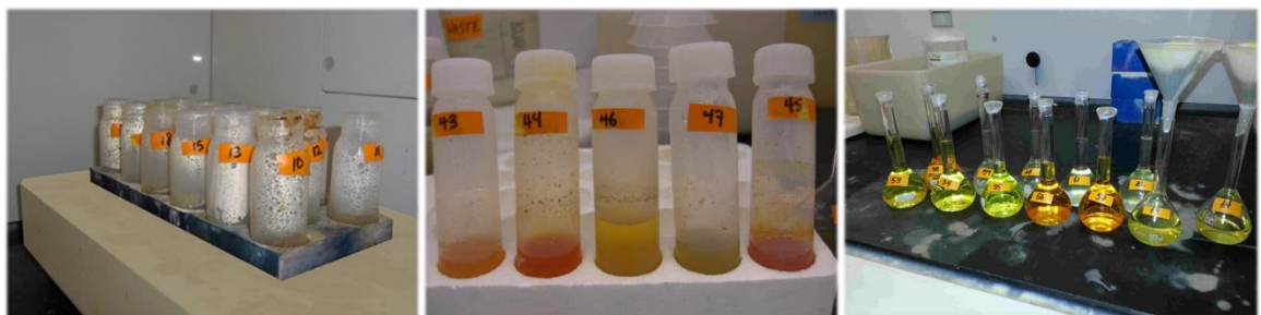
Figure 13: Digesting samples on heat block, cooling samples, filtered and filtering digested samples in 50 mL volumetric flasks
