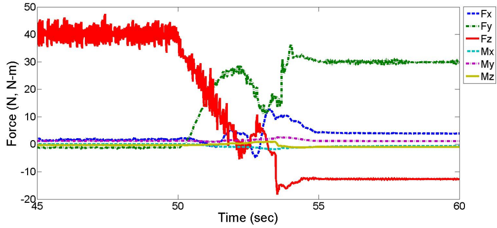
Figure 4.12: Total Impedance Force for Insertion
