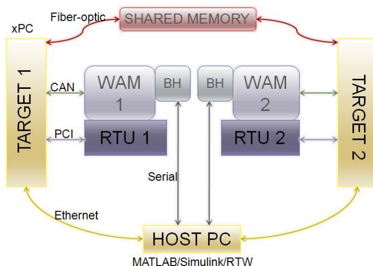
Figure 3.1: Workcell Diagram
