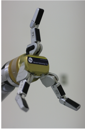
Figure 3.3: Barrett Hand
