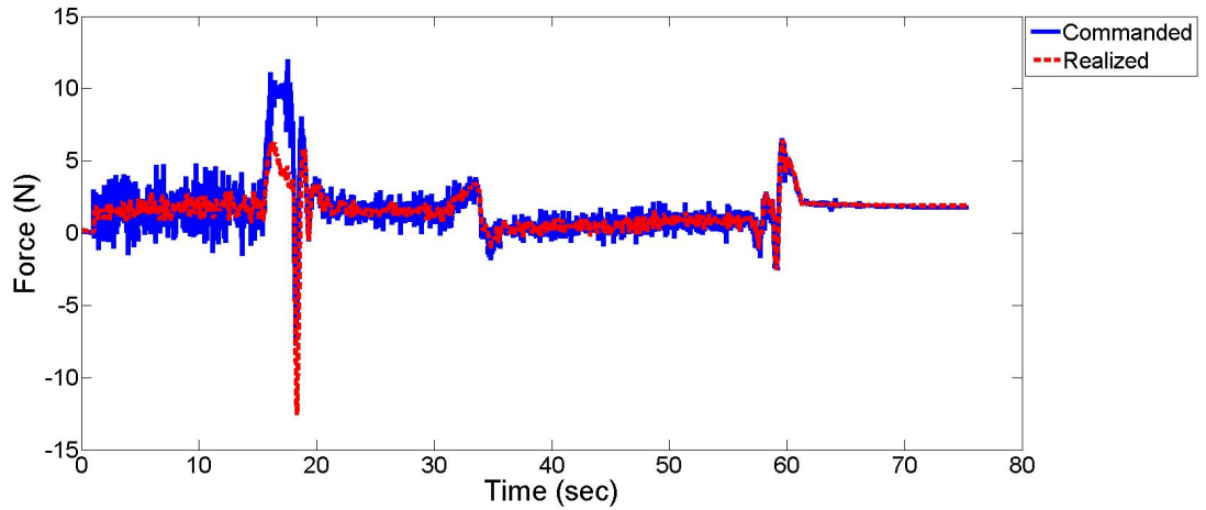
Figure 4.15: Commanded and Realized RTU Forces
