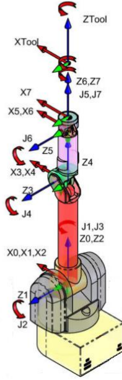
Figure 3.4: Frame Assignments for 7-dof WAM[1]
