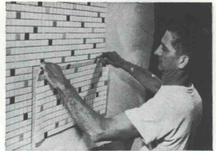
Here full sheets of back-mounted ceramics are hung in place. TILE-SET holds sheets without slippage. Allows ample open time for adjusting.
