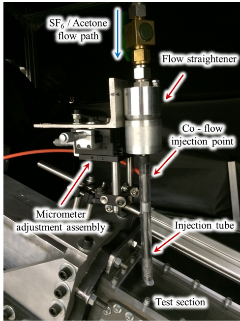
Figure 2.3: Image of the injector assembly, showing the flow path of the initial conditions. The ICs are first injected into a flow straightener before entering the injection tube, stabilized by a co-flow of air. This ensures the column of heavy gas remains a laminar jet through the test section. A micrometer adjustment assembly was added as a method of centering the jet with the exit hole on the bottom of the test section.
