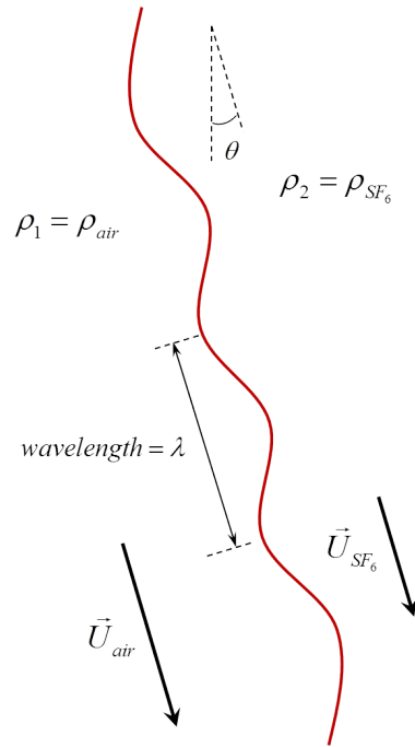
Figure 3.3: Modified schematic of the same perturbed interface as in Fig. 3.2, showing the inclined interface between the column of SF 6 and the surrounding air, where \theta is the angle of inclination from vertical. \vec{U}_{air} corresponds to the velocity of the light gas (air) moving down the interface, while \vec{U}_{SF_6} corresponds to the velocity of the heavy gas (SF 6 ). In this schematic, the velocity of the lighter gas is greater than the velocity of the heavy gas.
