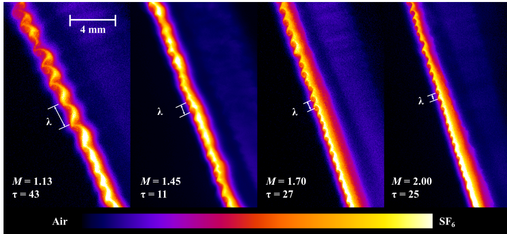
Figure 4.3: Comparison of KHI vortices at four different Mach numbers for a 30^\circ angle of inclination. Mach number increases from left to right: M = 1.13 , M = 1.45 , M = 1.70 , and M = 2.00 .
