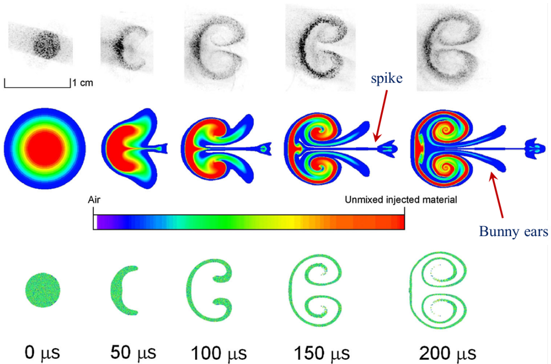
Figure 1.1: Comparison of experimental images (top) using glycol fog as a tracer, density contours generated by SHAMRC (middle) for pure \text{SF}_6 initial conditions, and particle distributions generated by SHAMRC with initial particle distribution taking the difference between \text{SF}_6 concentration and particle concentration into account [1].
