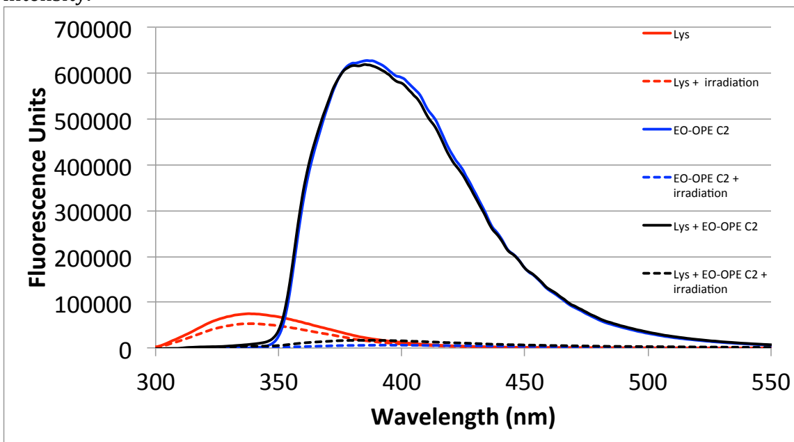
Figure 14: Fluorescence spectra of Lys at excitation 280 nm under various conditions. The intrinsic peak for proteins appears at 340 nm with EO-OPE c2 peaks appearing further into the red spectra. The protein alone exhibits a high fluorescence that is then reduced in the presence of the compound shown in red. The intensity of the compound over shadows that of the protein. However, similar results as with BSA occur for lysozyme.
