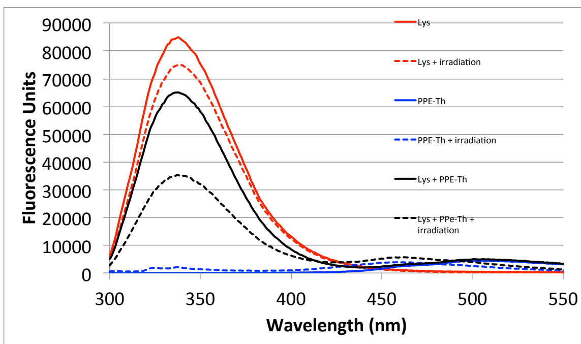
Figure 12: Fluorescence spectra of Lys at excitation 280 nm under various conditions. The intrinsic peak for proteins appears at 340 nm with PPE-DABCO peaks appearing further into the red spectra. The protein alone exhibits a high fluorescence that is then reduced in the presence of the compound shown in red. After irradiation there is blue spectral shift for the compounds and increased intensity. Irradiation also has an effect on lysozyme alone.
