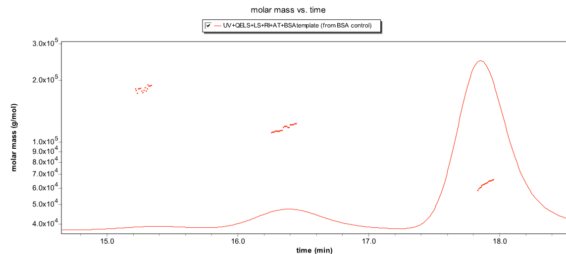
Figure 29: This is a molar mass vs time for the Dawn Heleos-II of BSA control. Displayed is the UV chromatograph collect form HPLC with the clusters showing mass. 100 \mu\text{g} of protein have been loaded to collect data. On this we have starting from the left trimer peak (182 kDa), dimer peak (117.3 kDa), and monomer peak (62.9 kDa) for BSA.
