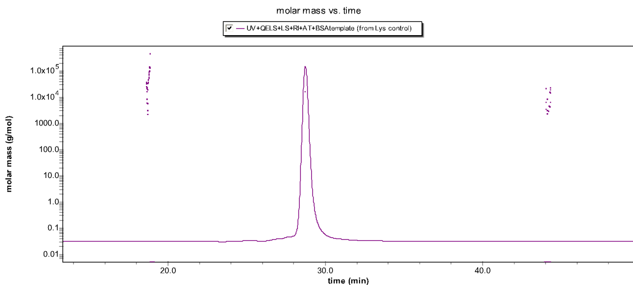
Figure 31: This is a molar mass vs time for the Dawn Heleos-II of Lysozyme control. Displayed is the absorbance data collect form HPLC with the clusters showing the mass distribution. 100 \mu\text{g} of protein have been loaded to collect data. There is a single peak for lysozyme the monomer peak (14.49 kDa).
