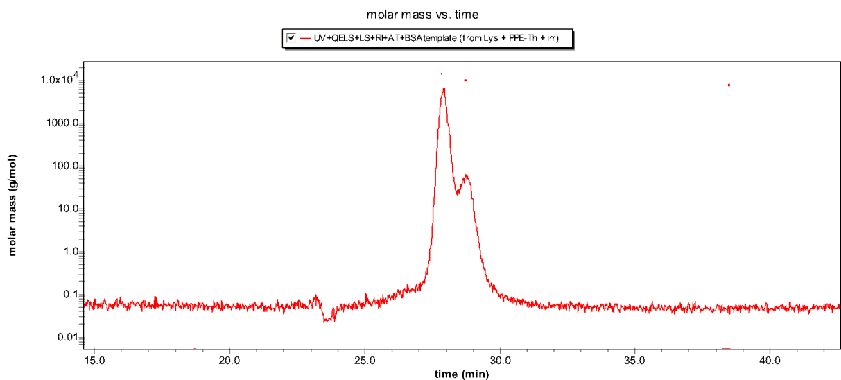
Figure 32: This is a molar mass vs time for the Dawn Heleos-II of Lysozyme with PPE-Th after irradiation. Displayed is the absorbance data collect from HPLC with the clusters showing the mass distribution. 100 \mu\text{g} of protein and 10 \mu\text{g} of PPE-Th have been loaded to collect data There are two peaks for lysozyme the monomer peak on the left (14.23 kDa) and smaller product at (10.16 kDa). This mass difference as before can be contributed to the interaction of PPE-Th and protein.
